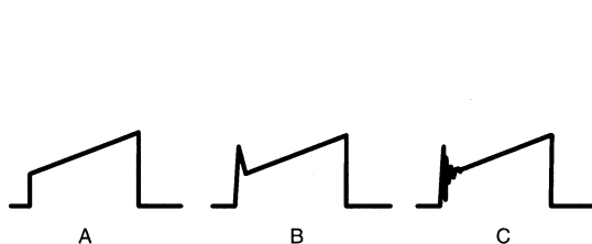
FIGURE 13. Current Waveforms
