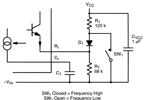
FIGURE 9. Frequency Shifting Using R_T Current Change
