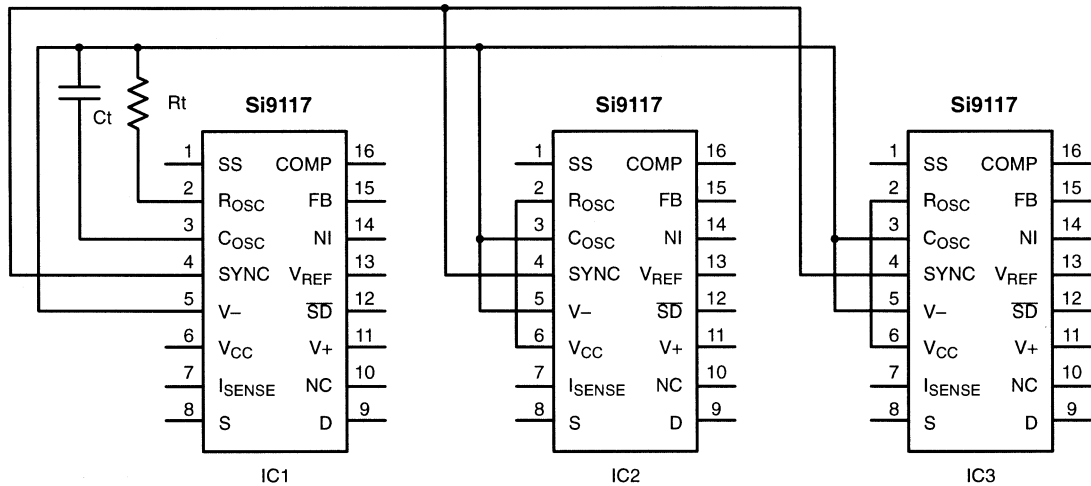
FIGURE 10. Oscillator Synchronization
