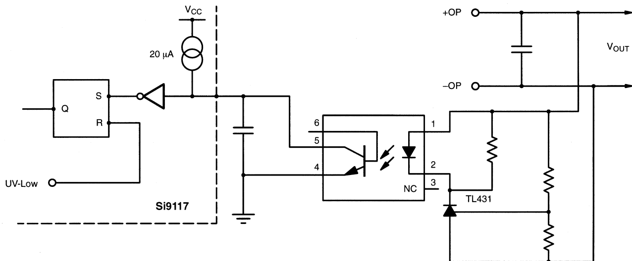
FIGURE 4. Shutdown
