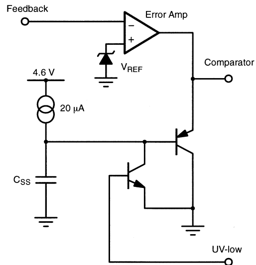
FIGURE 6. Soft-Start
