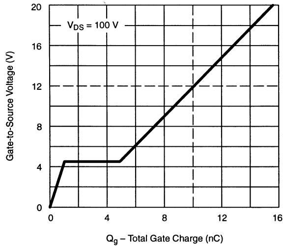
FIGURE 11. Si9117 Internal MOSFET Gate Change
