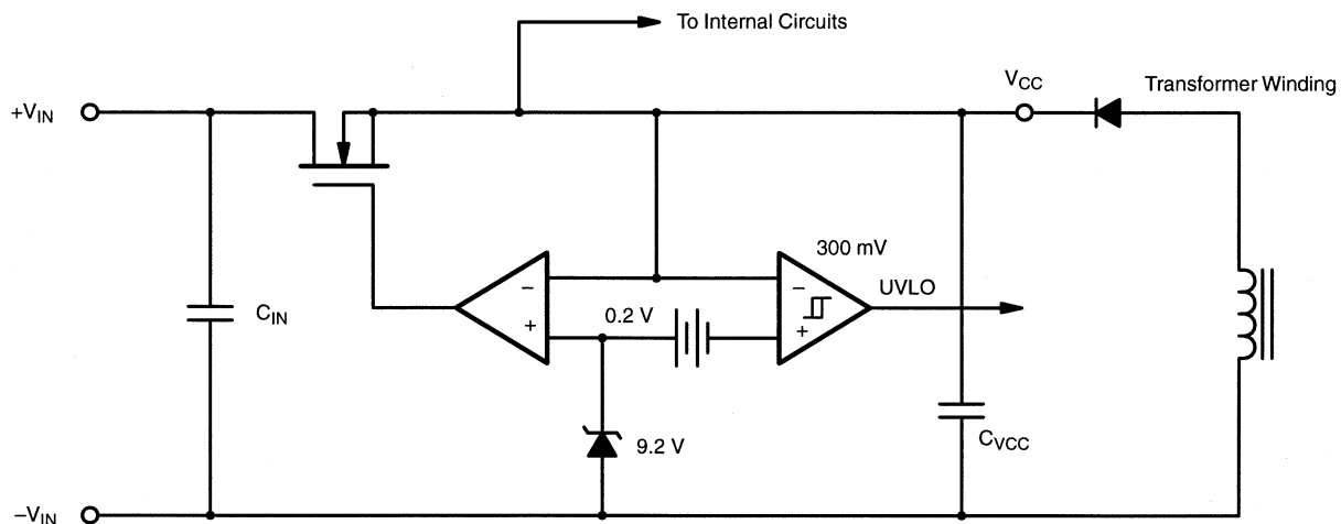
FIGURE 3. Start Circuit
