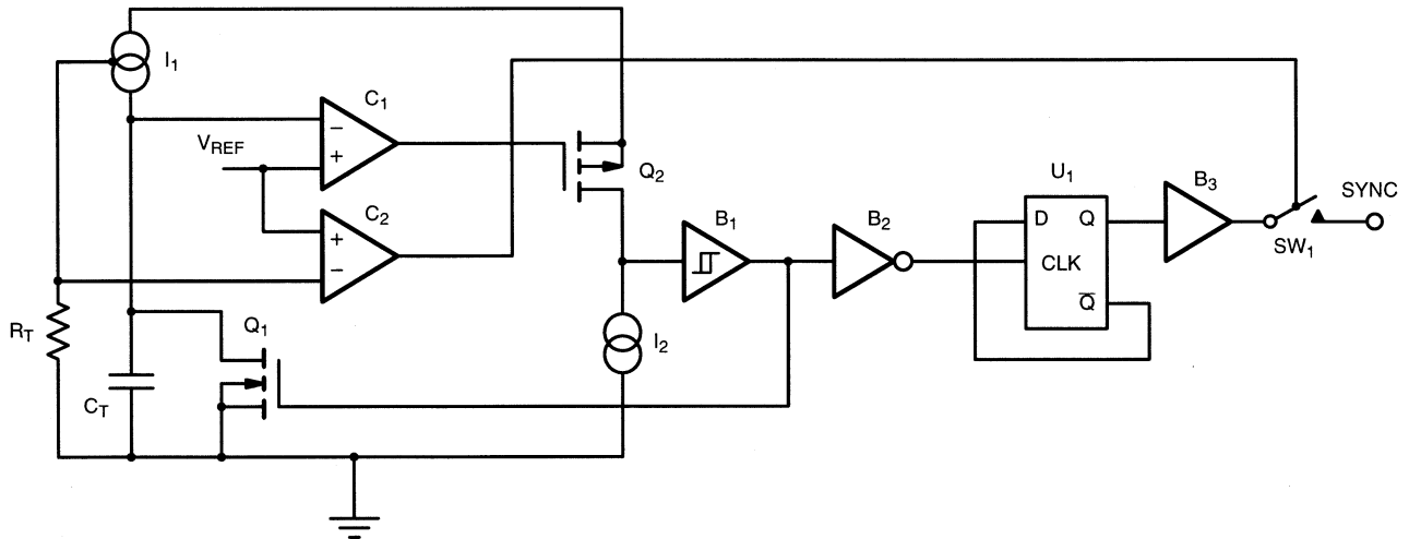
FIGURE 7. Oscillator
