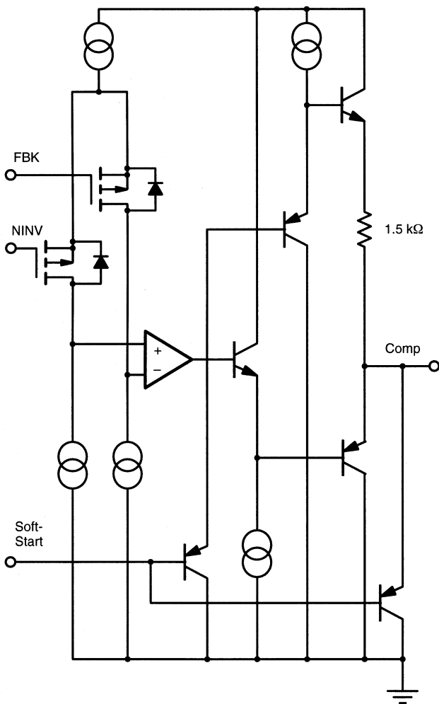
FIGURE 5. Operational Amplifier
