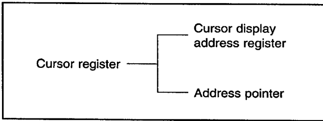
Figure 54. Cursor addressing
