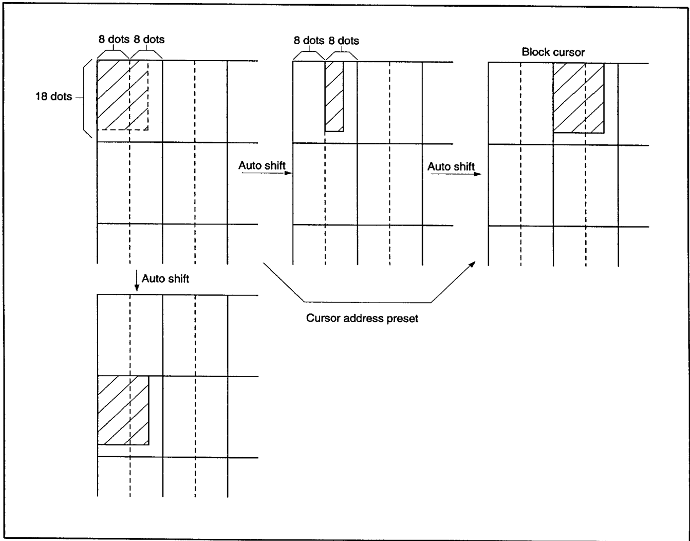
Figure 56. Cursor movement
