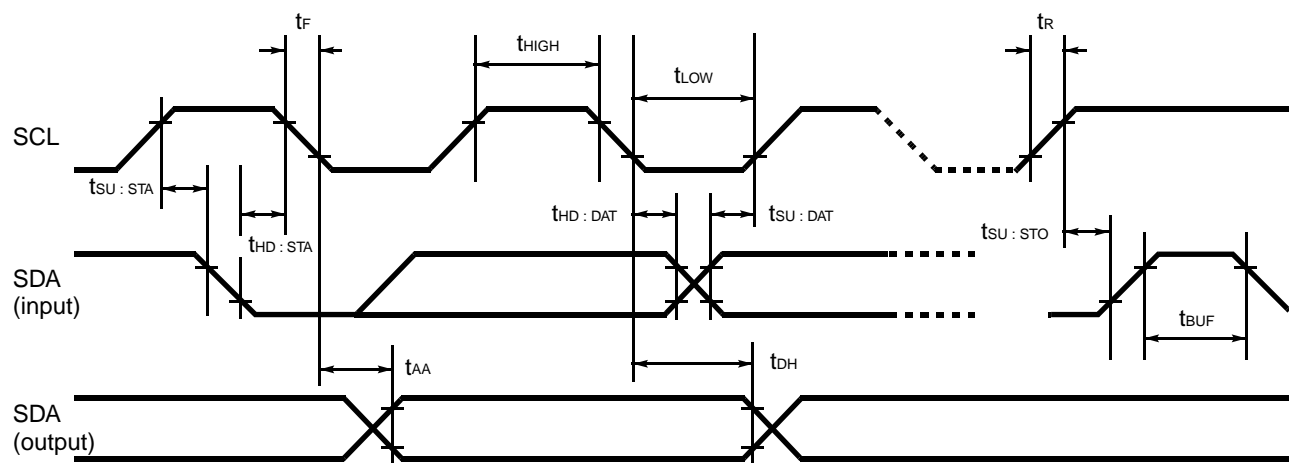
Fig. 6 – TIMING WAVEFORM
