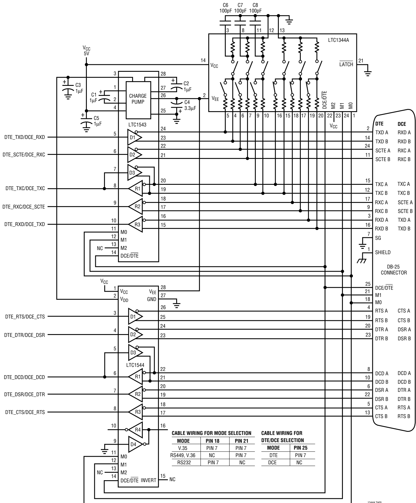
Cable Selectable Multiprotocol DTE/DCE Port with DB-25 Connector
