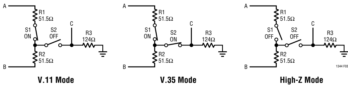
Figure 3. LTC1344A Modes
