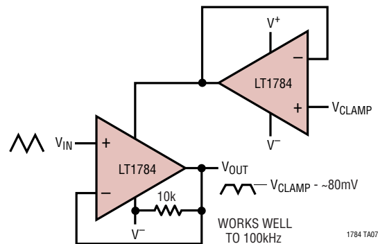
Adjustable Clamp
