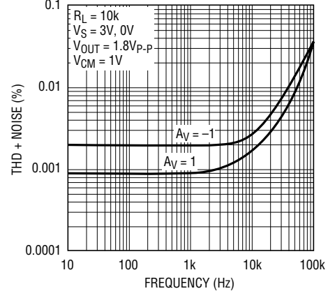
Total Harmonic Distortion + Noise vs Frequency
