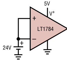
INPUT OVERVOLTAGE
