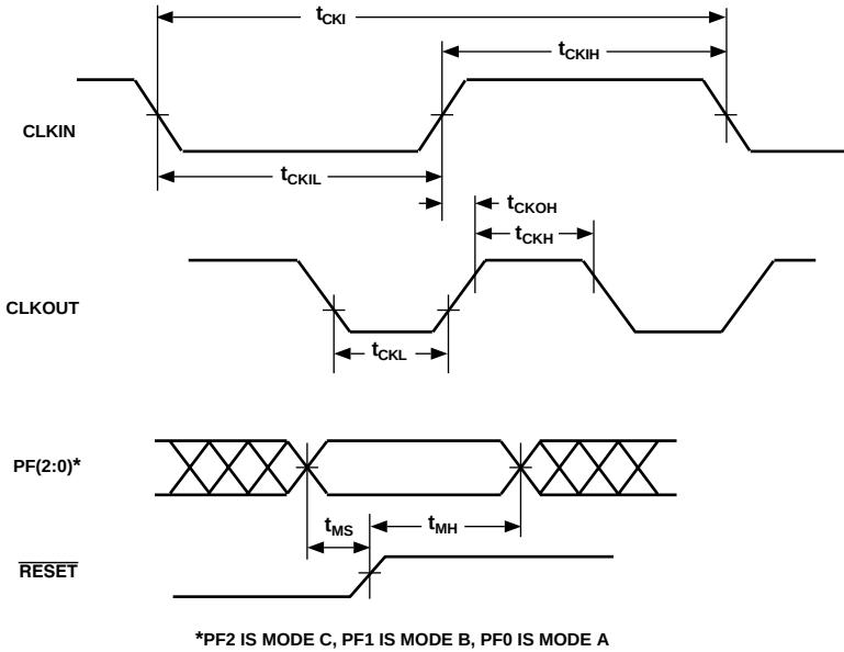
Figure 8. Clock Signals
