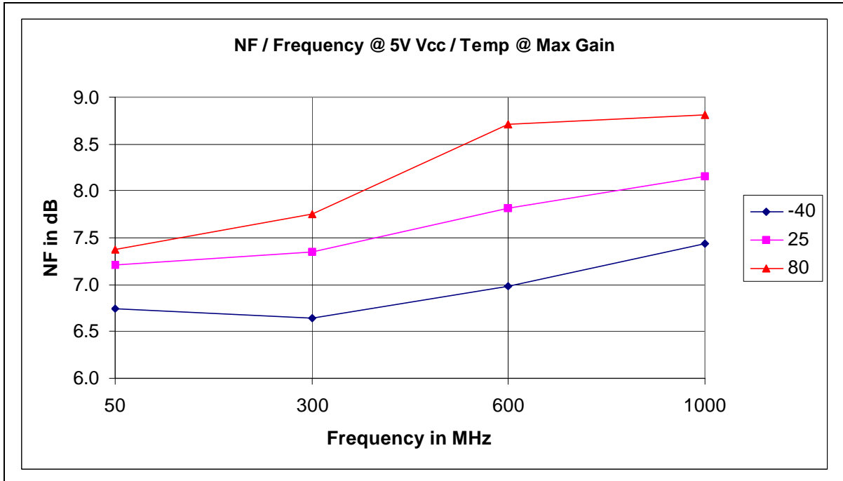
Figure 33 - Typical NF / Frequency @ 5V Vcc / Temp @ Max Gain
