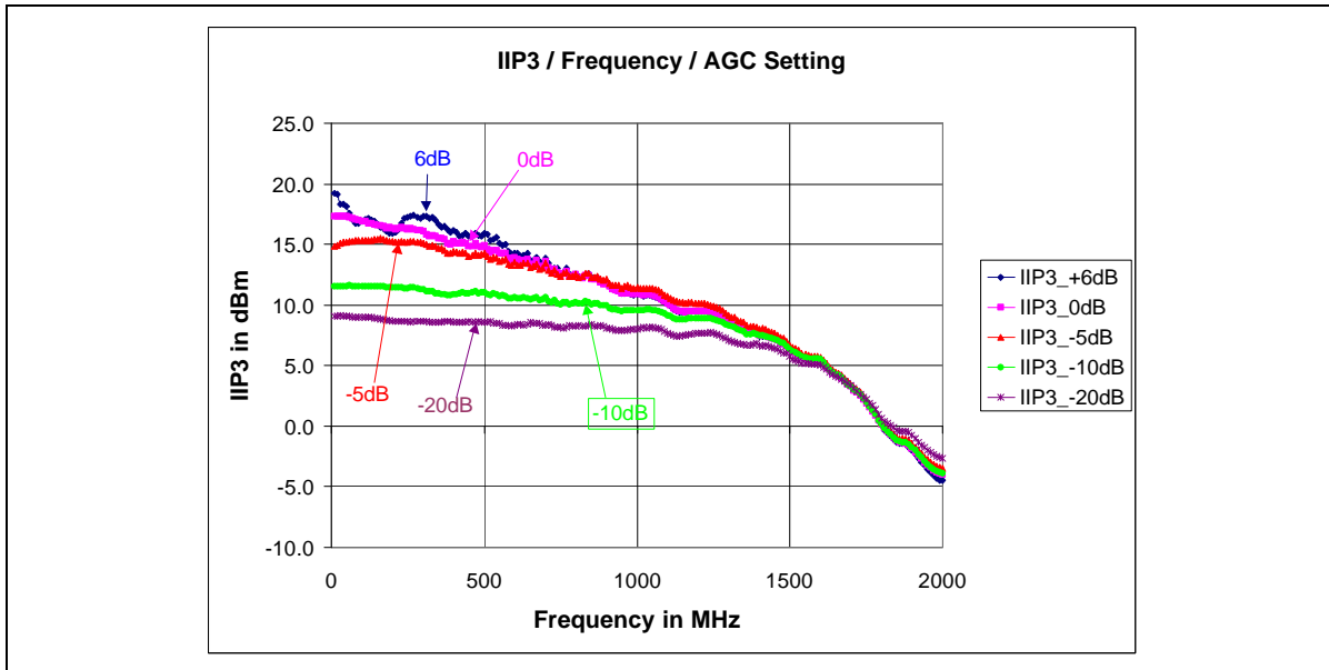
Figure 30 - Typical IIP3 @ Max Gain Differential / Frequency
