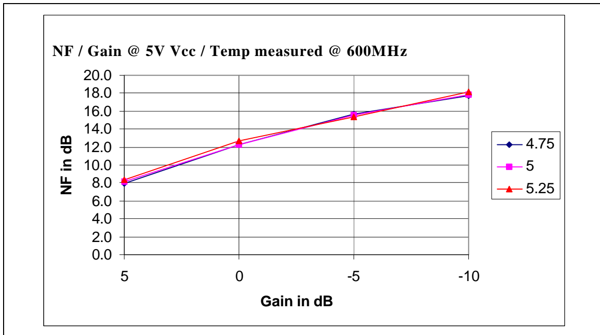
Figure 34 - Typical NF / Gain @ 5V Vcc / Temp measured @ 600MHz
