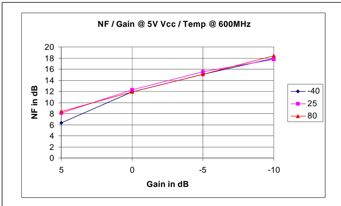
Figure 35 - Typical NF / Gain @ 25C / Vcc measured @ 600MHz
