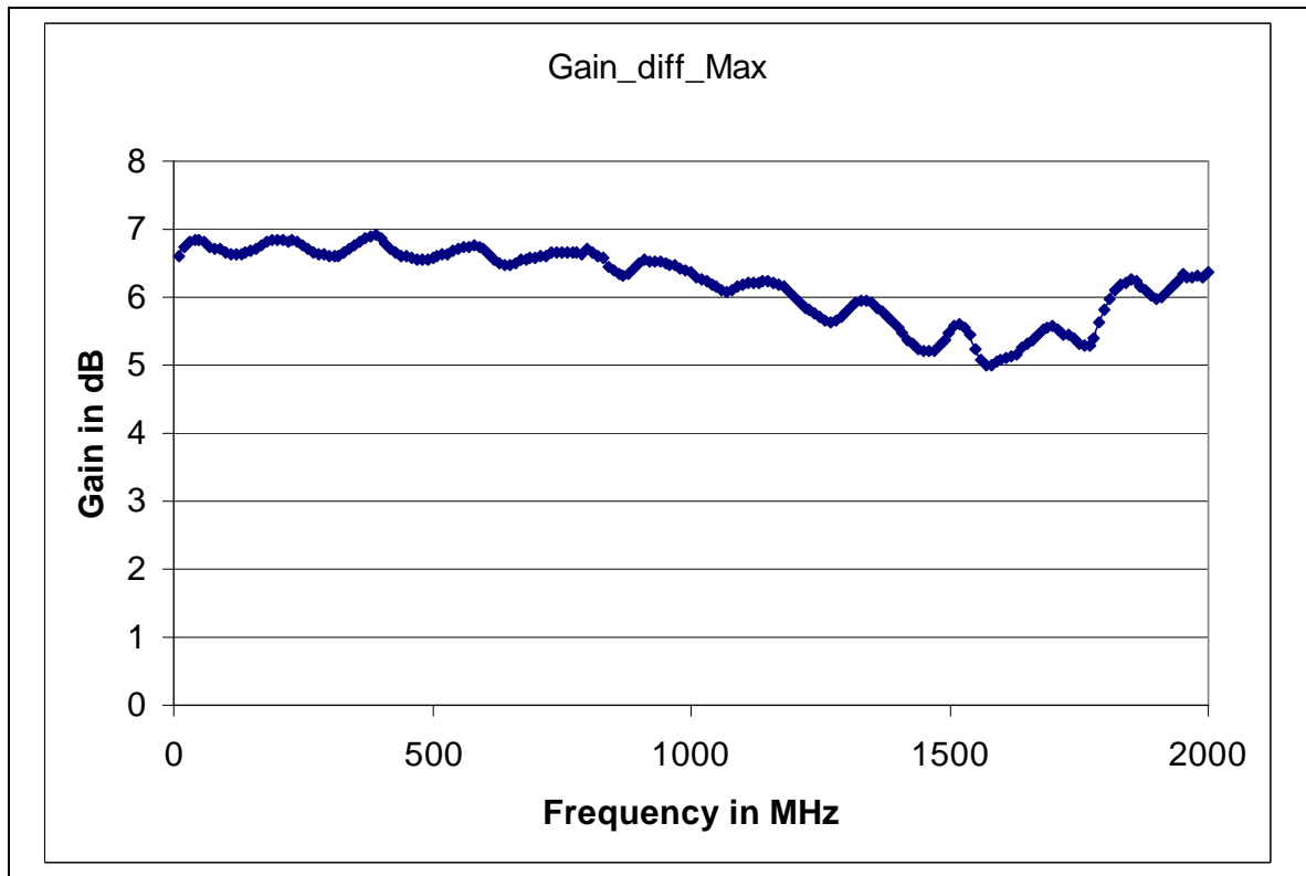
Figure 10 - Typical Diff Max Gain / Frequency
