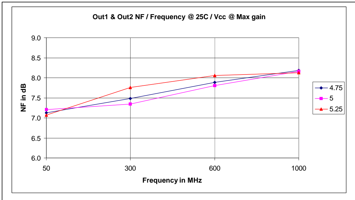
Figure 32 - Typical NF / Frequency @ 25C / Vcc @ Max Gain
