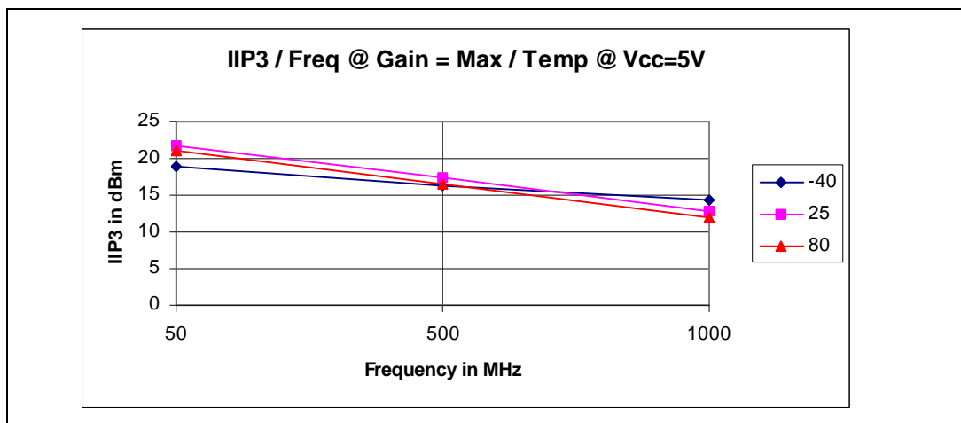
Figure 27 - Typical Out1, Out2 & Out3 IIP3 / Frequency @ Gain = Max / Temp @ 5V Vcc
