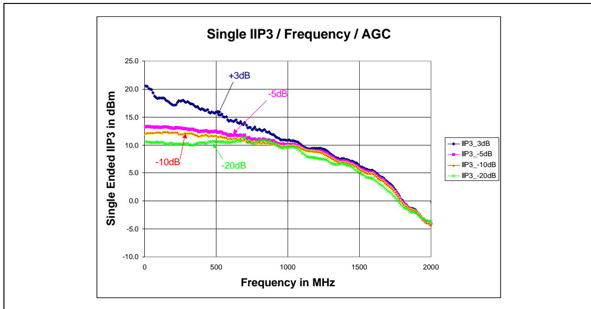
Figure 31 - Typical IIP3 Single Ended / Frequency / AGC
