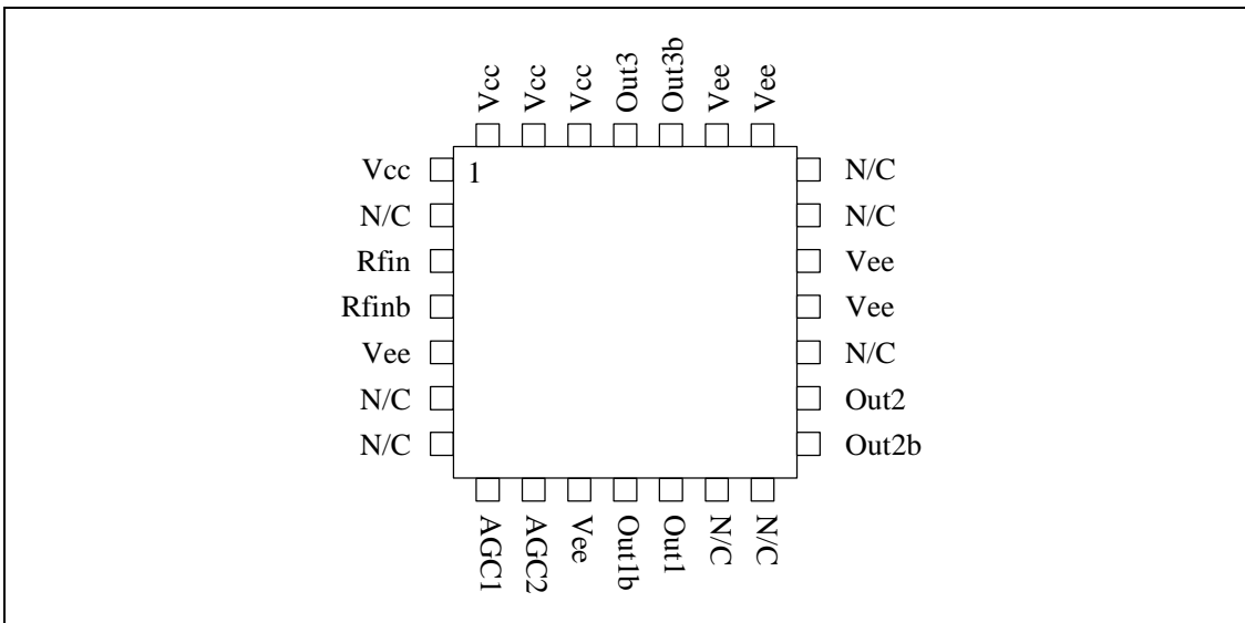
Figure 2 - Pin Diagram
