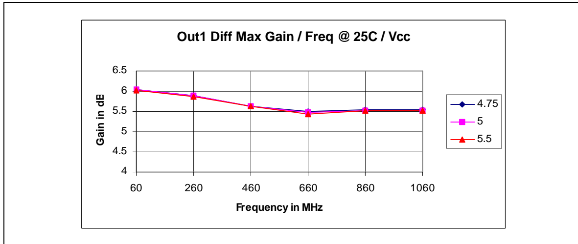
Figure 6 - Typical Ch1&2 Diff Gain / Freq / Vcc @ 25C
