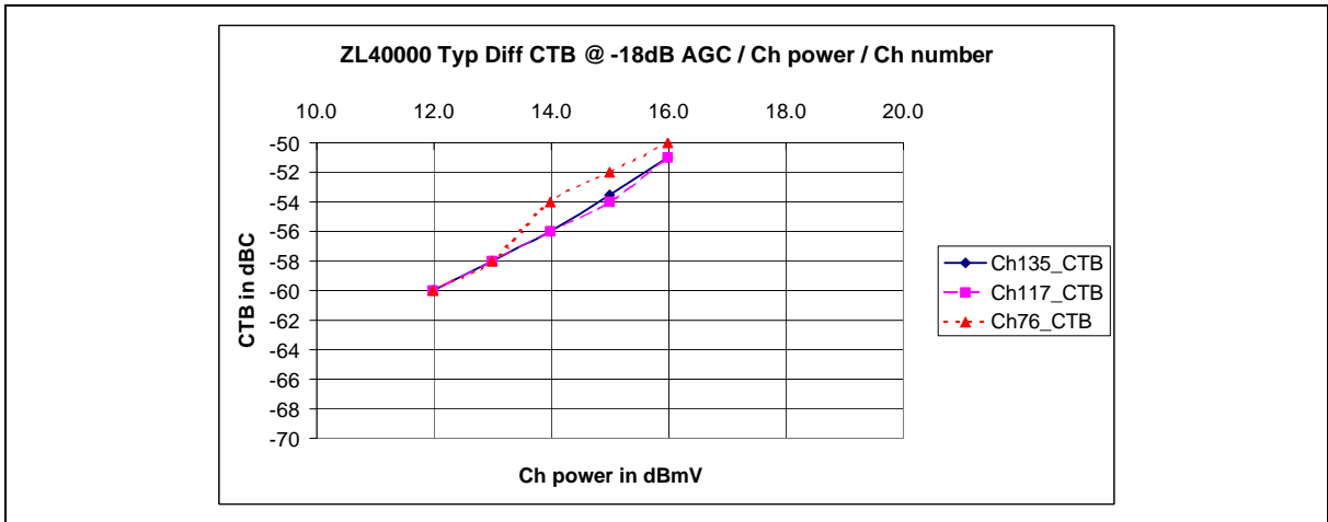
Figure 40 - CH136, CH117 and CH76 @ 850MHz, 745MHZ and 499MHz respectively
