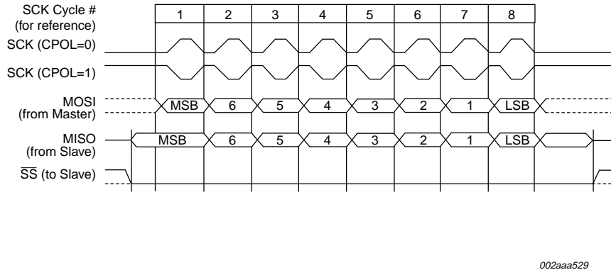
Fig 17. SPI transfer format with CPHA = 0.
