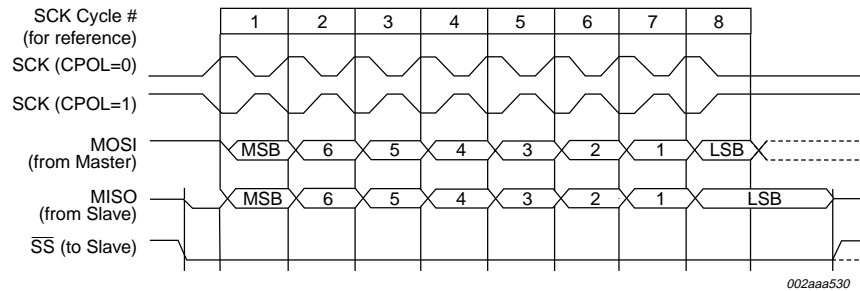
Fig 18. SPI transfer format with CPHA = 1.
