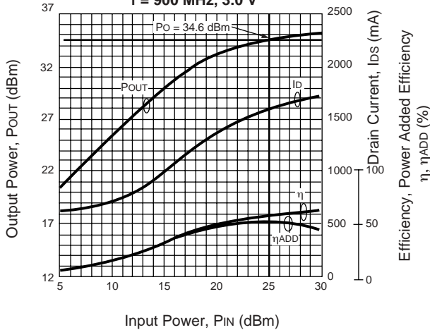
OUTPUT POWER, DRAIN CURRENT, EFFICIENCY AND POWER ADDED EFFICIENCY vs. INPUT POWER f = 900 MHz, 3.0 V
