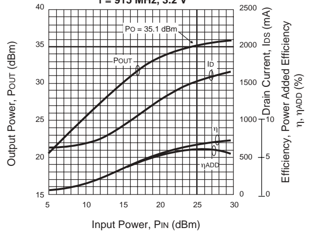
OUTPUT POWER, DRAIN CURRENT, EFFICIENCY AND POWER ADDED EFFICIENCY vs. INPUT POWER f = 915 MHz, 3.2 V
