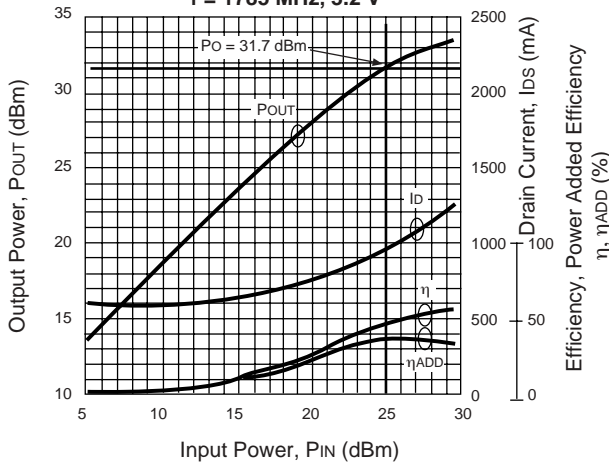
OUTPUT POWER, DRAIN CURRENT, EFFICIENCY AND POWER ADDED EFFICIENCY vs. INPUT POWER f = 1785 MHz, 3.2 V
