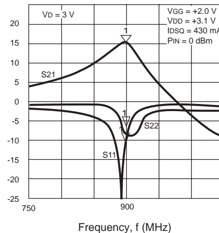
SMALL SIGNAL (0 dBm Input) GAIN AND RETURN LOSS
