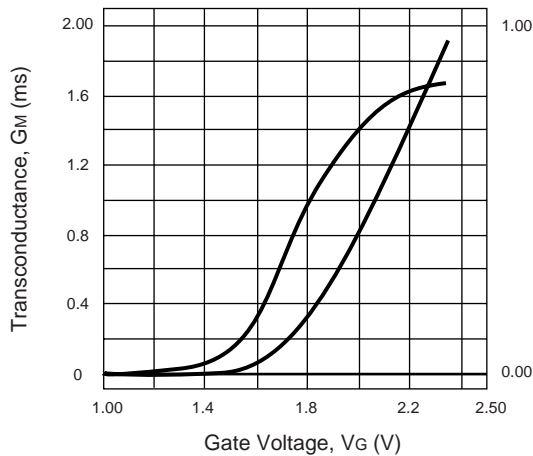
TRANSCONDUCTANCE AND DRAIN CURRENT vs. GATE VOLTAGE
