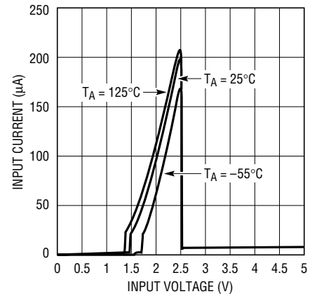
LTC1258-2.5 Input Current vs Input Voltage in Dropout
