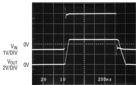
Output Overdrive Recovery
