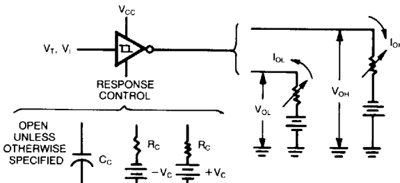
Figure 1 — V_{T+}, V_{T-}, V_{OH}, V_{OL}
