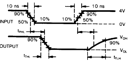
VOLTAGE WAVEFORMS
