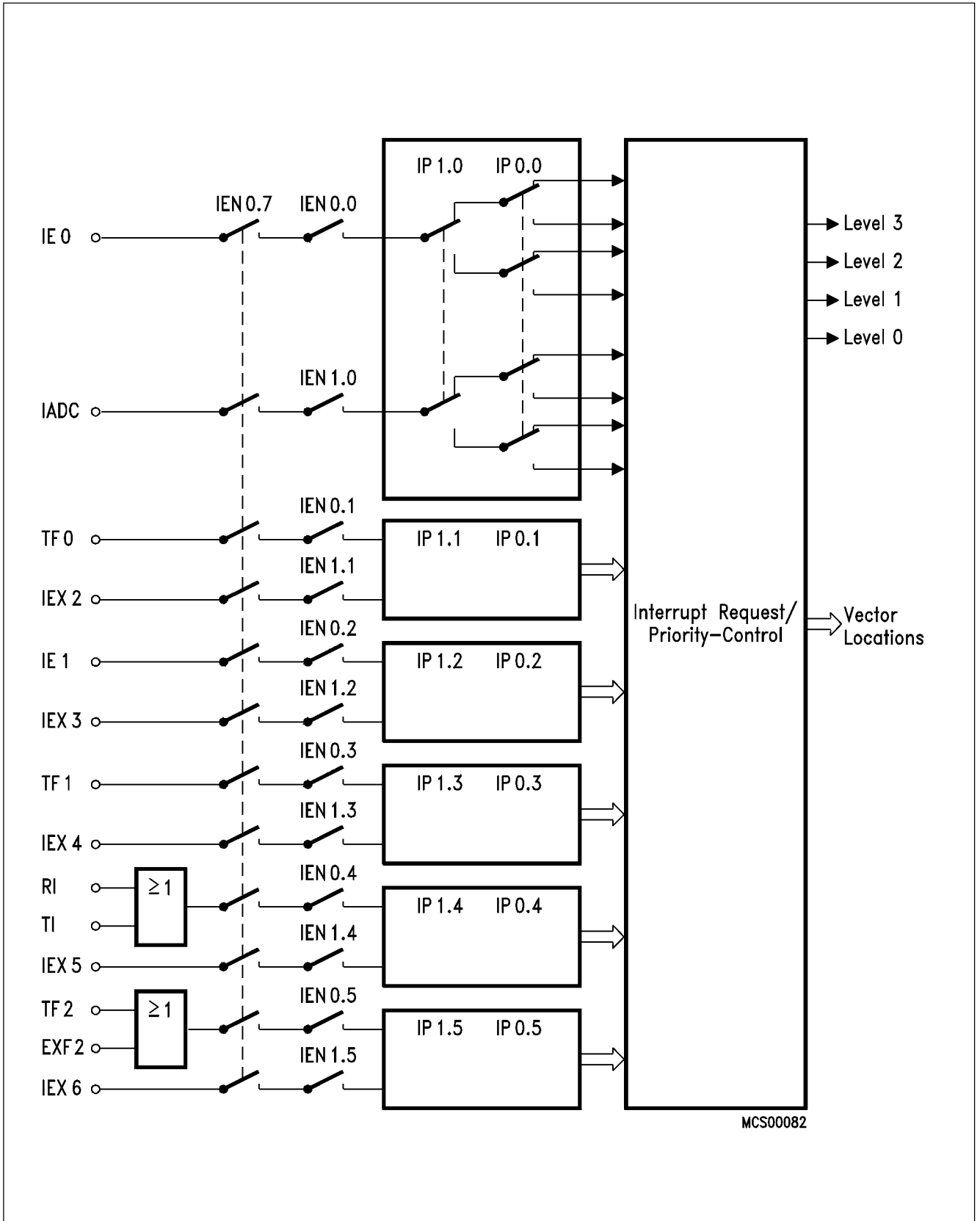
Figure 6 Interrupt Priority Level Structure
