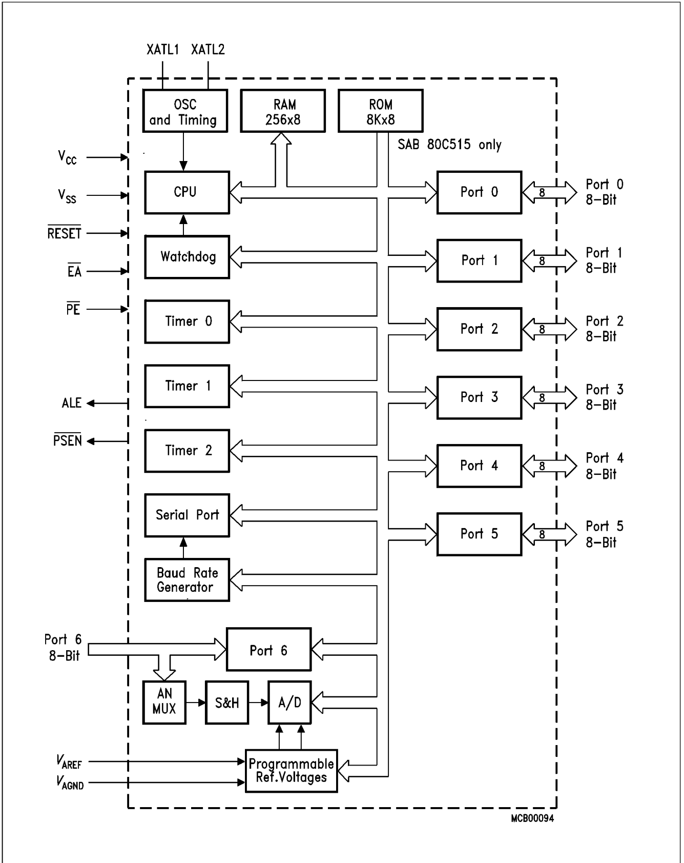
Figure 1 Block Diagram
