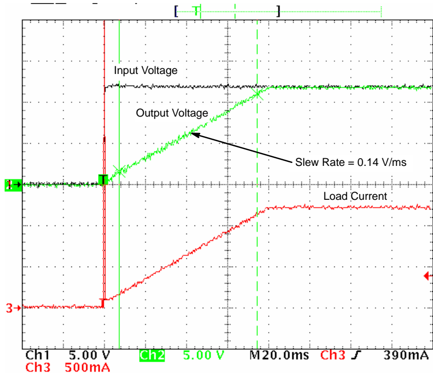
Figure 4. Turn-on Waveforms for a Resistive Load of 10 \Omega ( C_{dV/dt} = 1 \mu\text{f} )
