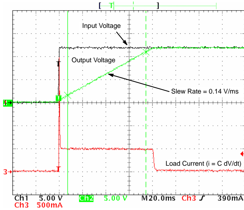
Figure 5. Turn-on Waveforms for a Load Capacitance of 3,300 \mu\text{f} ( C_{dV/dt} = 1 \mu\text{f} )
