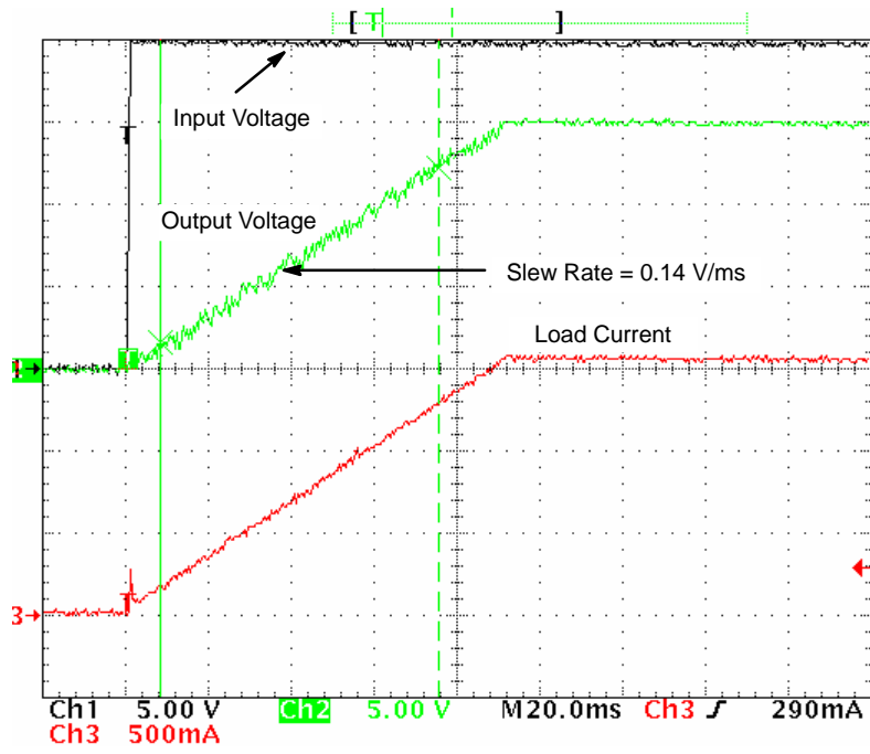
Figure 6. Turn-on Waveforms for an Overvoltage Condition (10 \Omega Resistive Load)
