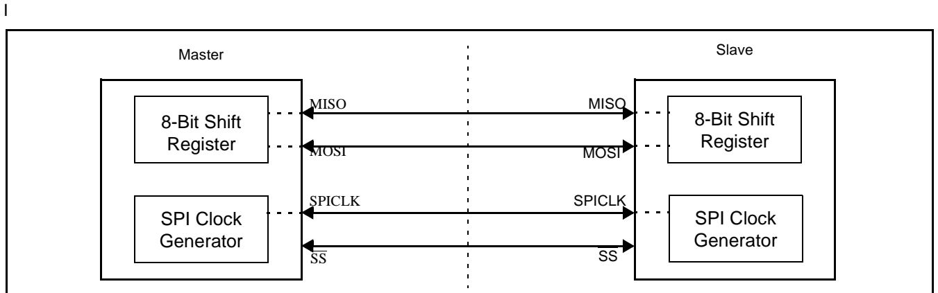
Figure 16: SPI dual device configuration, where either can be a master or a slave.
