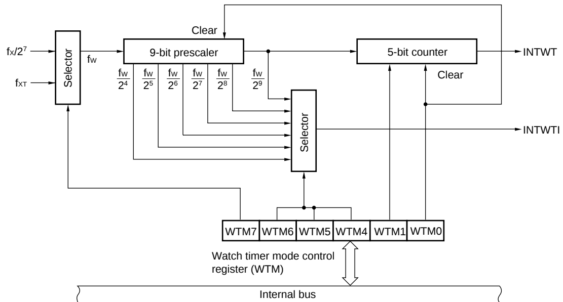
Figure 5-18. Watch Timer Block Diagram
