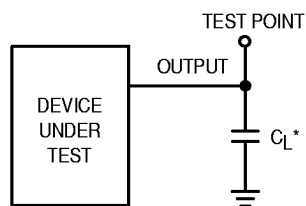
Figure 4. Test Circuit
