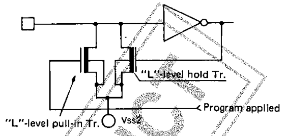
Fig. 4 Input configuration of S1-4, M1-4
