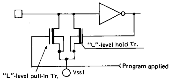
Fig. 1 Input configuration of S1-4, M1-4
