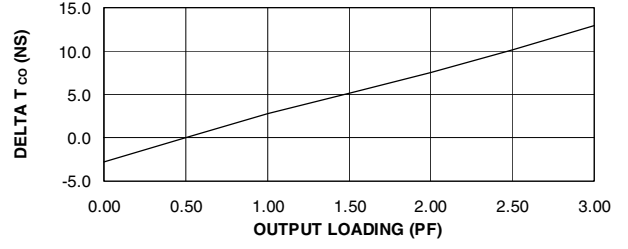
22LV10CZ/CQZ DELTA T_{CO} VS. OUTPUT LOADING
