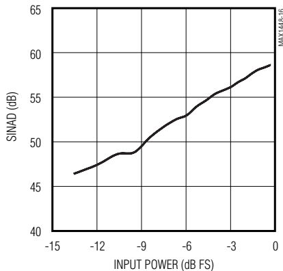
SIGNAL-TO-NOISE PLUS DISTORTION vs. INPUT POWER ( f_{IN} = 20MHz )
