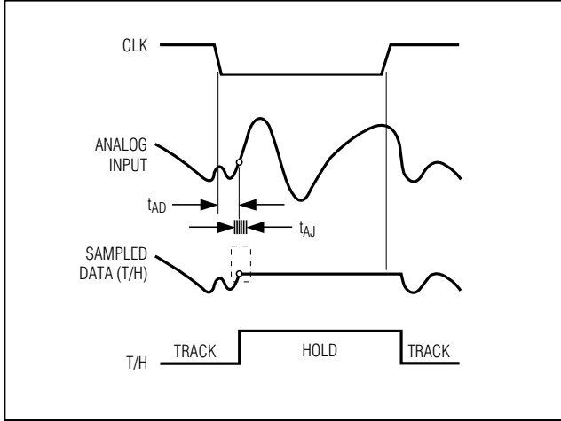
Figure 10. Track-and-Hold Aperture Timing
