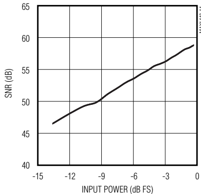
SIGNAL-TO-NOISE RATIO vs. INPUT POWER ( f_{IN} = 20MHz )
