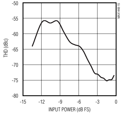
TOTAL HARMONIC DISTORTION vs. INPUT POWER ( f_{IN} = 20MHz )
