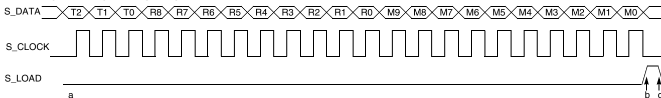
Figure 4: Serial Programming Timing Diagram
