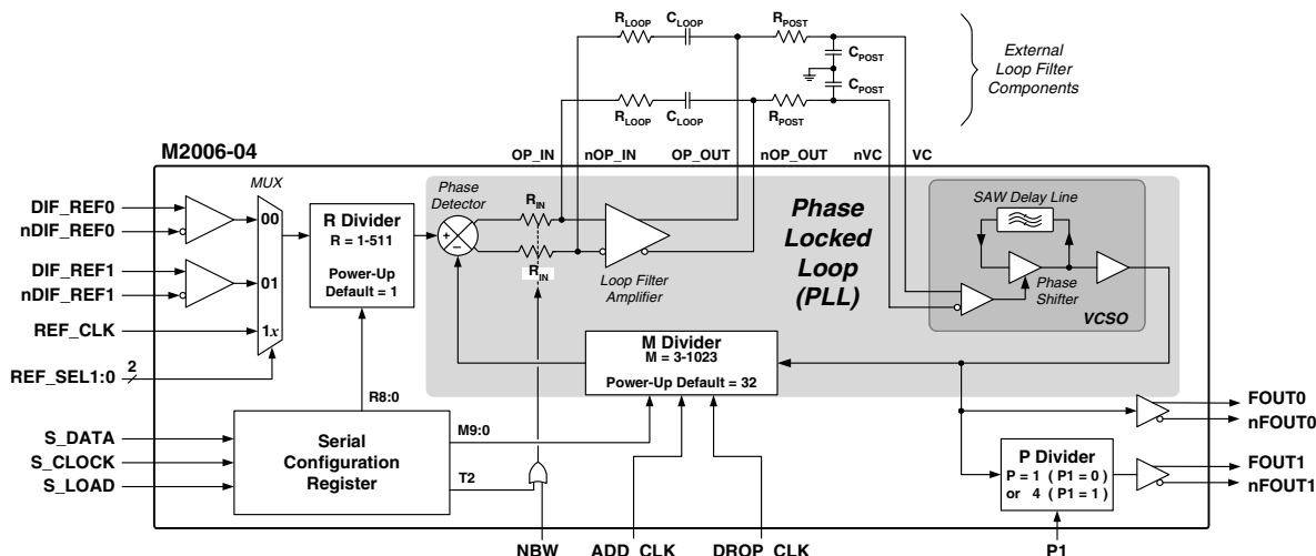
Figure 3: Detailed Block Diagram
