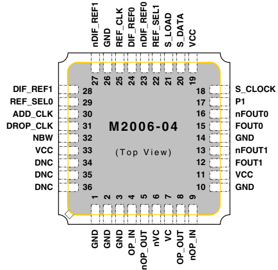
Figure 1: Pin Assignment
