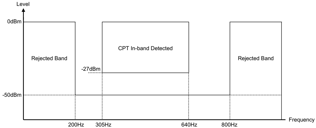
Call progress tone frequency band illustration
