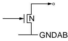
Fig. 3-18: Output pins RSW1, RSW2
