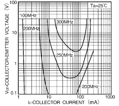
Fig.9 Gain bandwidth product
