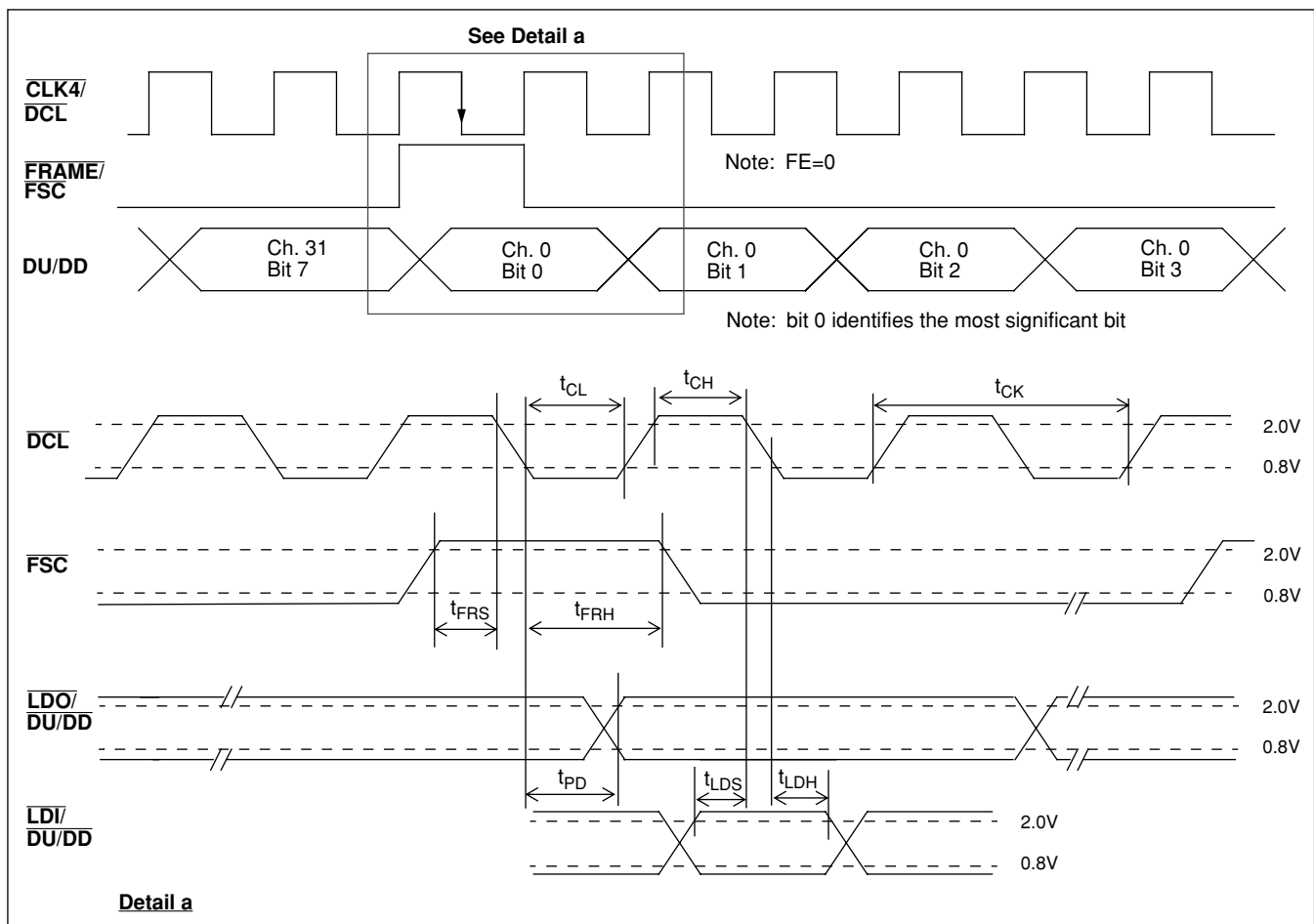
Figure 20 - GCI Timing
