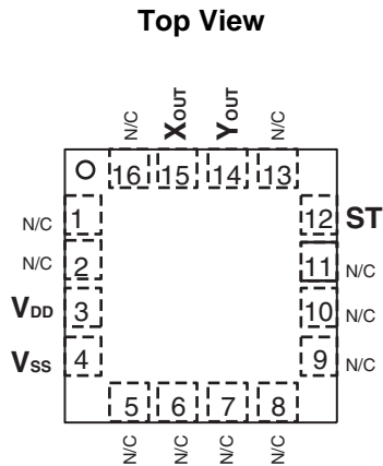
Figure 3. Pinout Description
