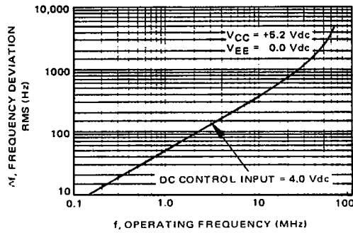
FIGURE 4 — RMS NOISE DEVIATION versus OPERATING FREQUENCY
