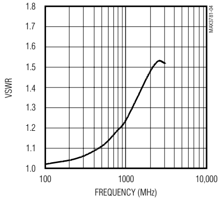
INPUT VSWR (BY SIMULATION)
