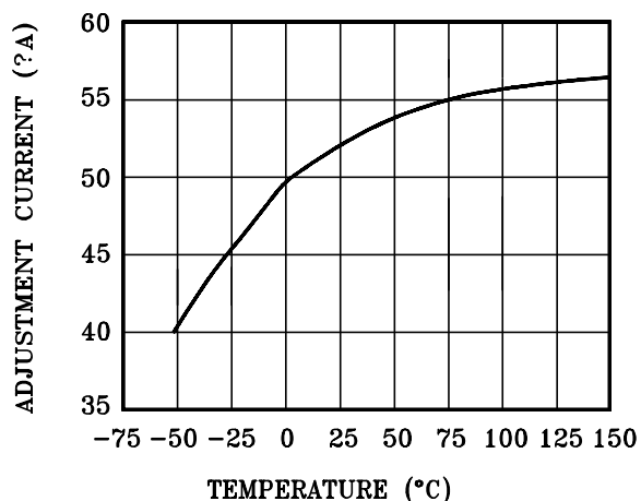
Adjustment Current
