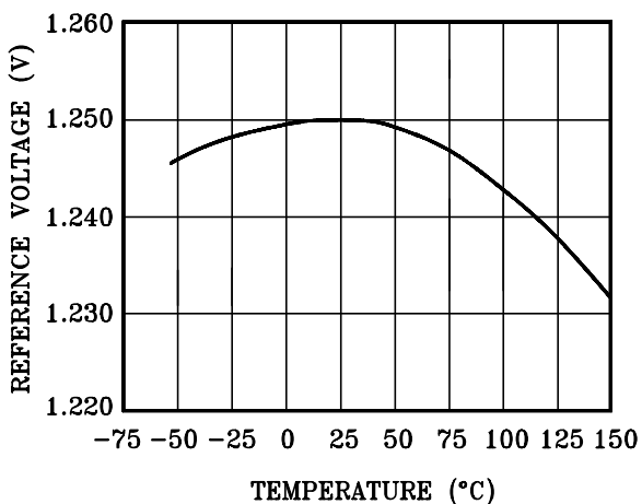
Temperature Stability
