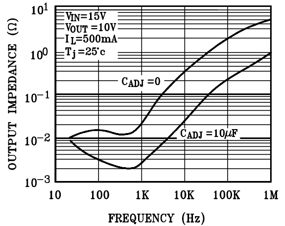
Output Impedance
