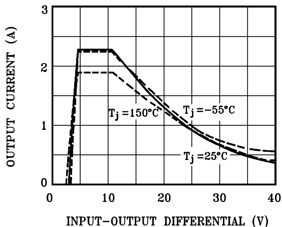
Current Limit
