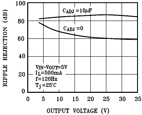
Ripple Rejection
