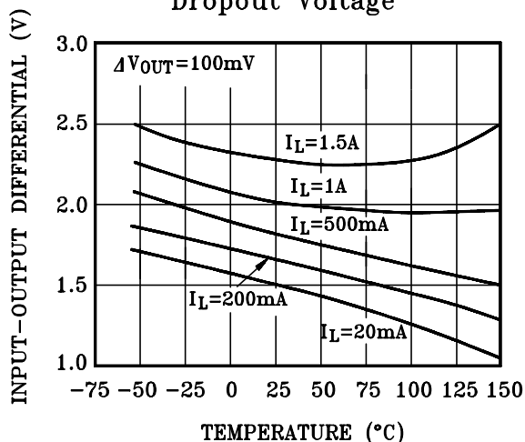
Dropout Voltage
