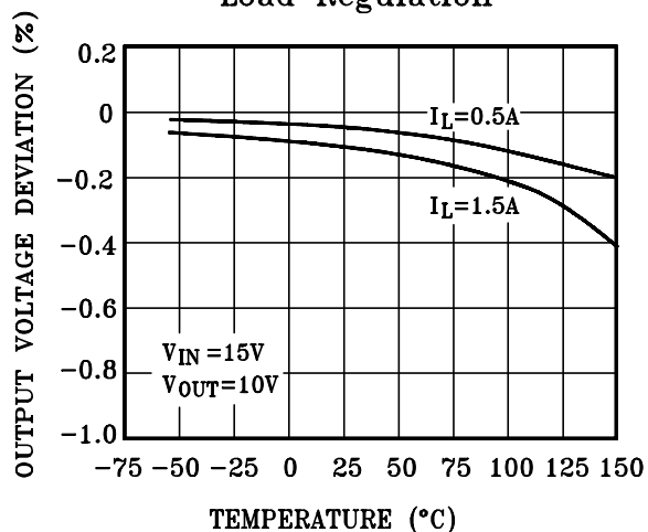
Load Regulation
