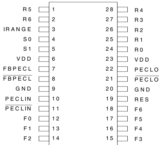
28-pin (150 mil) SSOP
