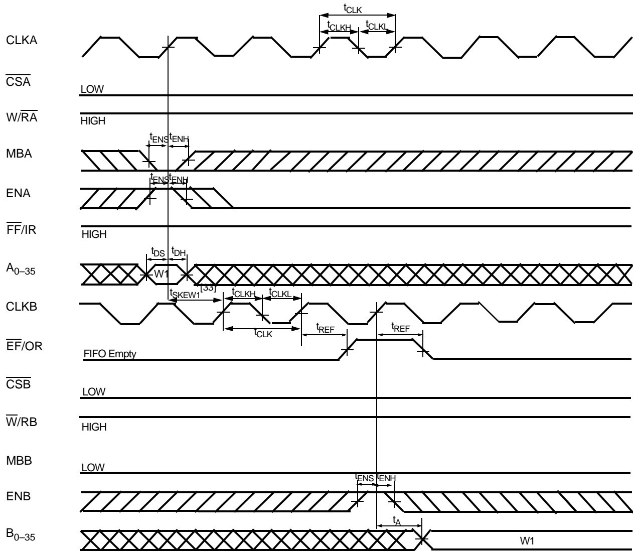
\overline{EF} Flag Timing and First Data Read Fall Through when FIFO is Empty (CY Standard Mode) [31]
