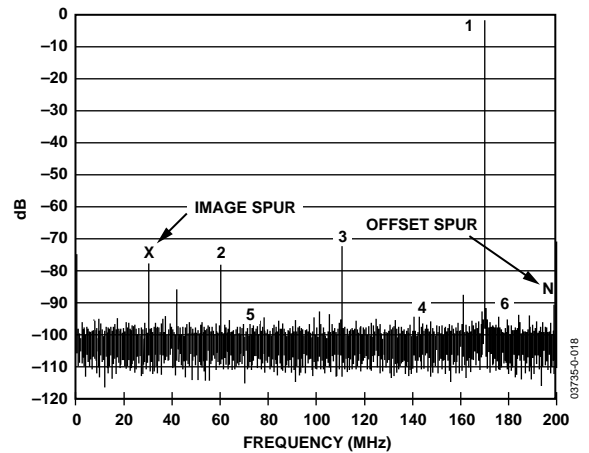
Figure 19. AD12400 with AFB Digital Post Processing
