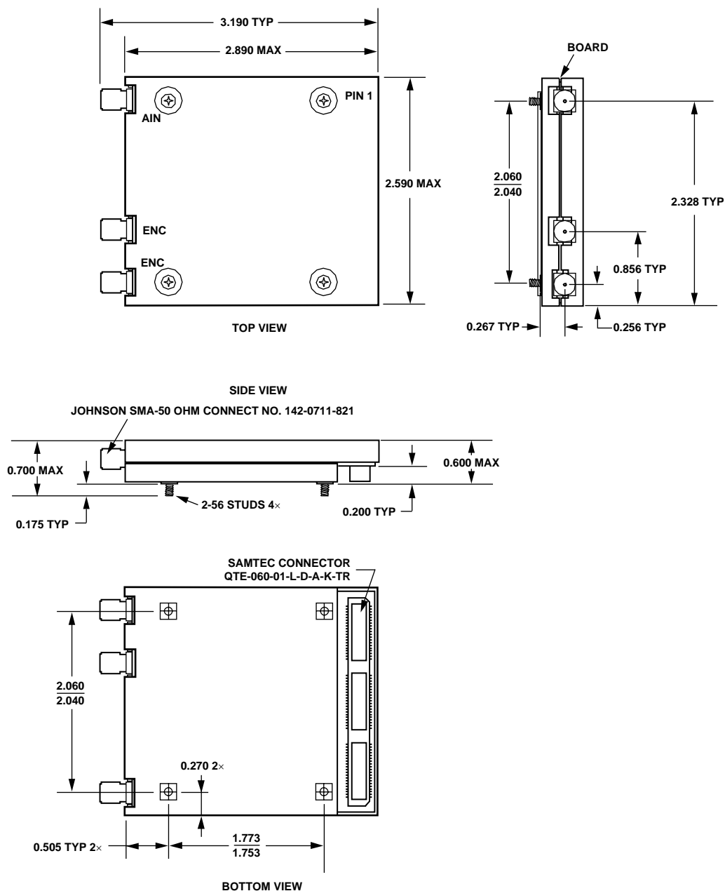
Figure 38. Outline Dimensions Dimensions shown in inches Tolerances: 0.xx = ±10 mils 0.xxx = ±5 mils
