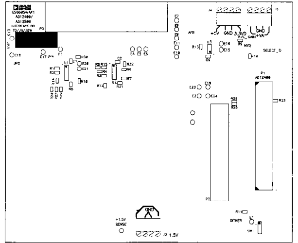
Figure 32. Top Silkscreen
