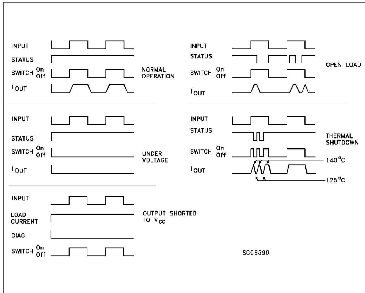
Figure 1: Waveforms
