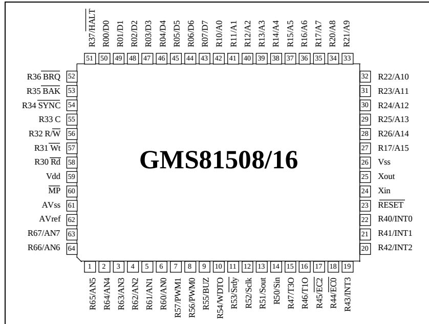
64 QFP
