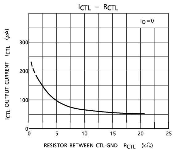
Fig.4 I_{CTL} - R_{CTL}
