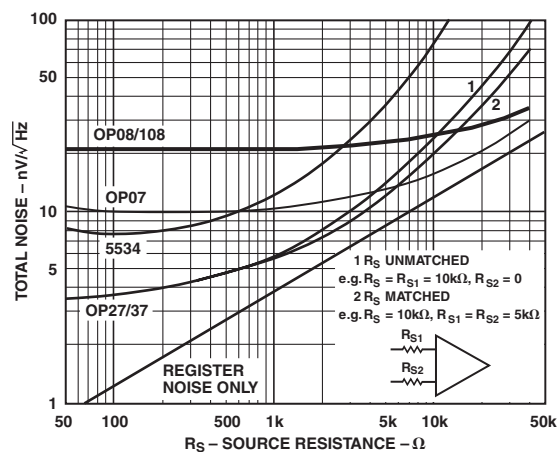
Figure 7. 10 Hz Noise vs. Source resistance (Includes Resistor Noise)
