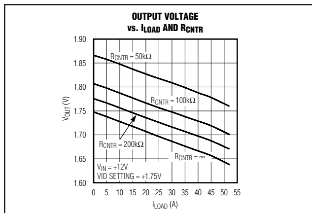
Figure 4. Output Voltage vs. I LOAD and RCNTR
