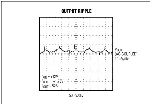
Figure 7. Output Ripple
