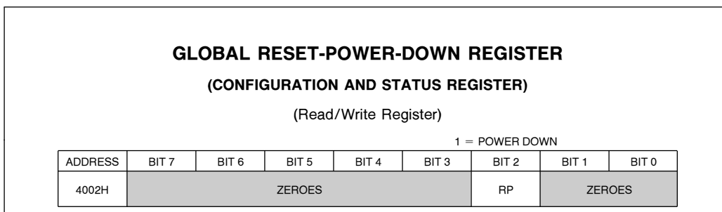
Figure 6. GLOBAL RESET-PWRDWN REGISTER (PCMCIA). The RP Bit Enables Reset PowerDown of All Flash Memory Devices.
