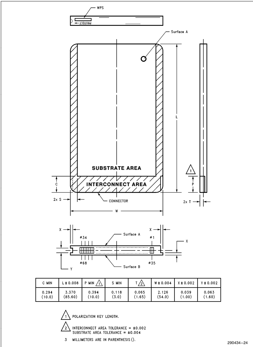
Figure 19. Series 2 Flash Memory Card Package Dimensions
