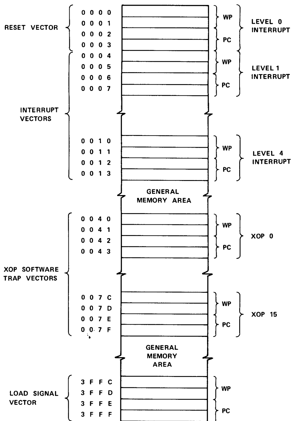
FIGURE 2 – MEMORY MAP
