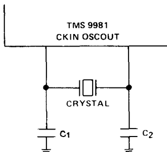
FIGURE 13 – CRYSTAL OSCILLATOR CIRCUIT
