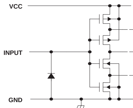
Input (SCLK)
