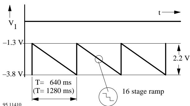
Figure 3. Ramp diagram without external circuit
