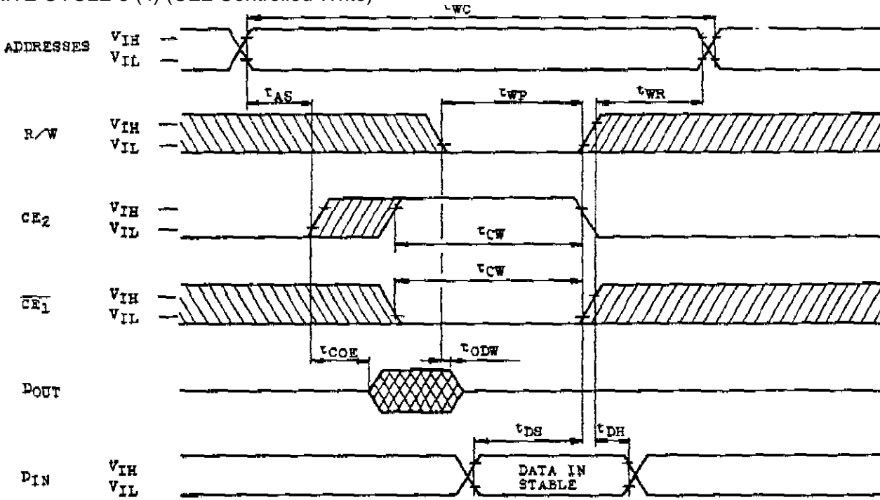
WRITE CYCLE 3 (4) ( \text{CE2} Controlled Write)
