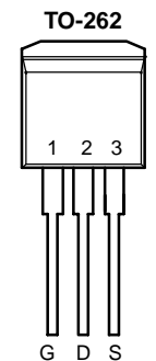
Top View SUV85N03-04P
