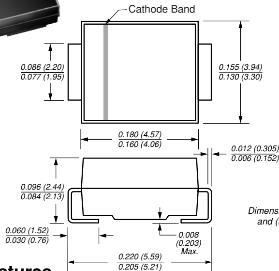
DO-214AA (SMB)
