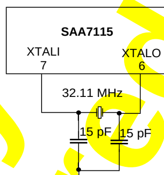
(1c) With fundamental quartz. Crystal load = 8 pF
