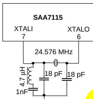
(2a) With 3rd harmonic quartz.
