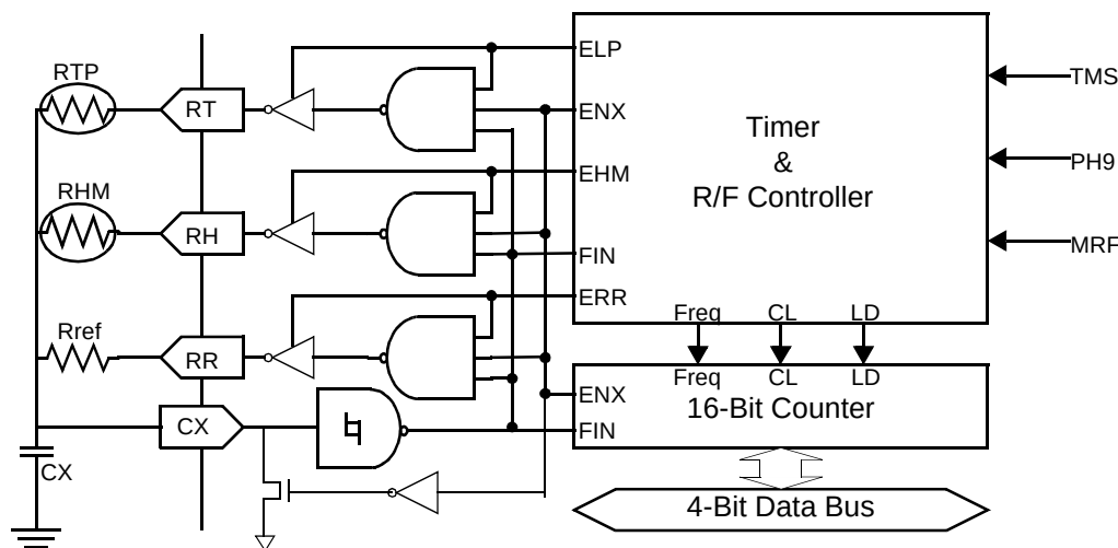
FIGURE 1. R to F Converter Diagram
