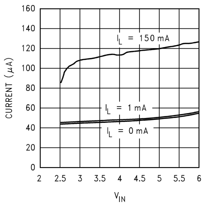
Ground Current vs V_{IN} @ -40^\circ C
