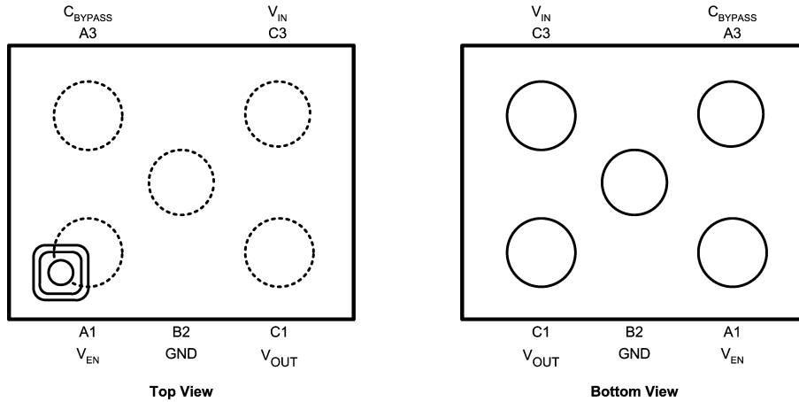
micro SMD, 5 Bump Package
