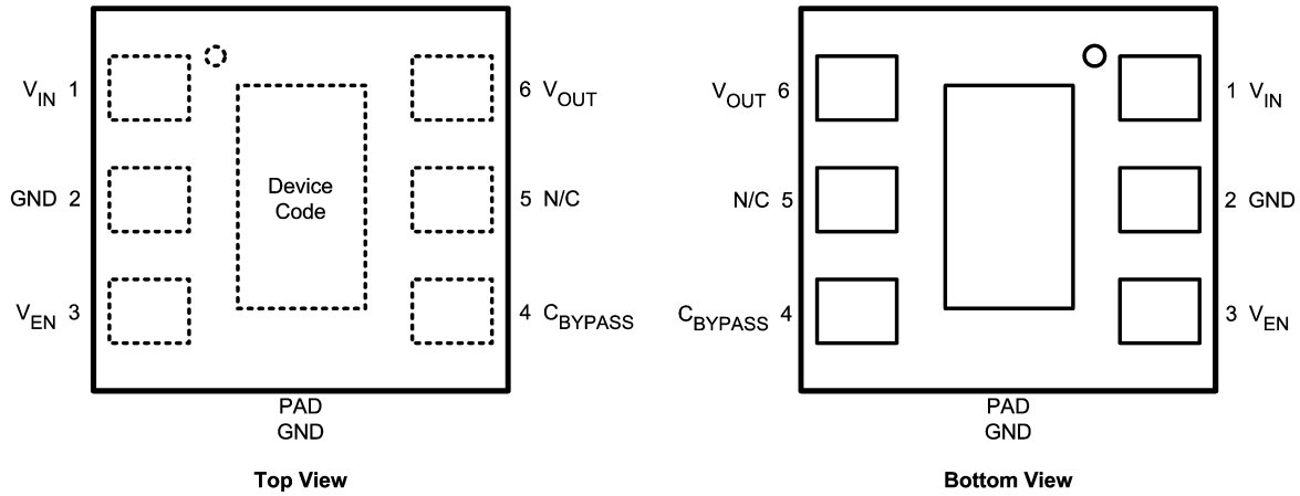
LLP-6 Package (SOT23 footprint)
