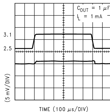
Line Transient Response (1.5V V_{OUT} )
