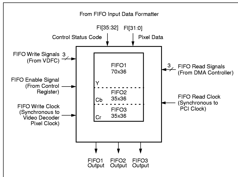
Figure 23. Data FIFO Block Diagram
