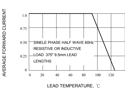
Fig. 1-FORWARD CURRENT DERATING CURVEE
