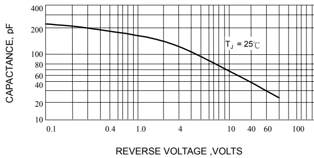
Fig. 4-TYPICAL JUNCTION CAPACITANCE
