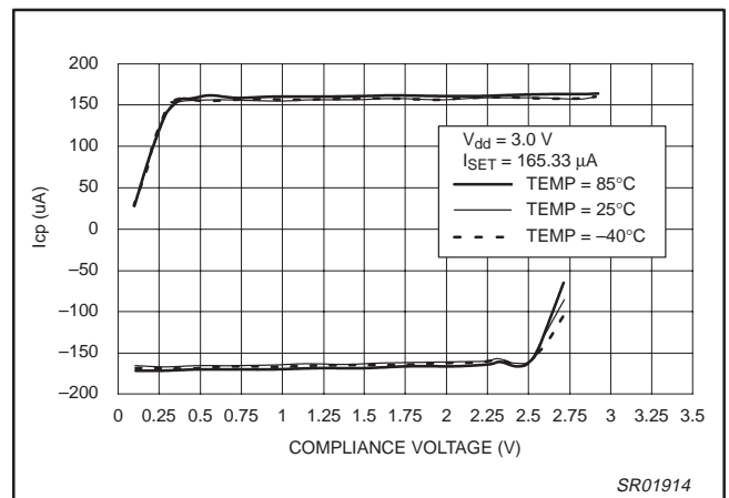
Figure 13. Php Charge Pump Output vs. Temperature (CP = 1; V DD = 3.0 V; I SET = 165.33 μA)
