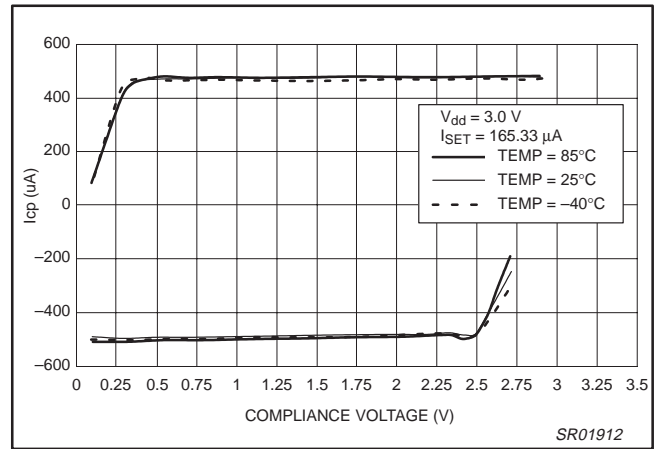
Figure 11. Php Charge Pump Output vs. Temperature (CP = 0; V DD = 3.0 V; I SET = 165.33 μA)
