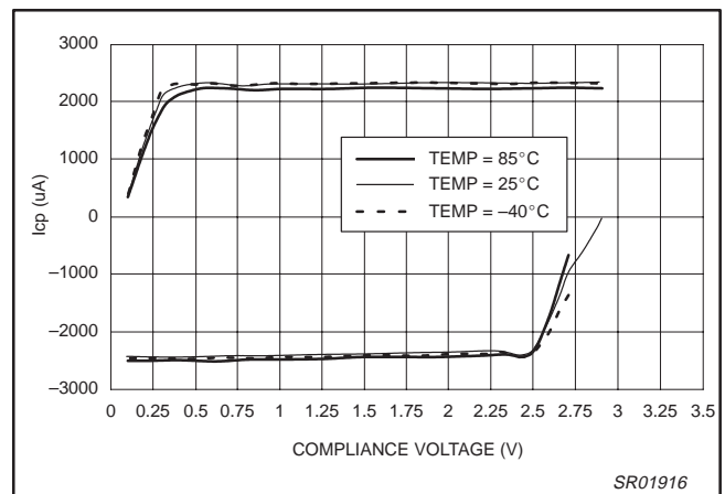
Figure 15. Php-su Charge Pump Output vs. Temperature (CP = 0; V DD = 3.0 V; I SET = 165.33 μA)
